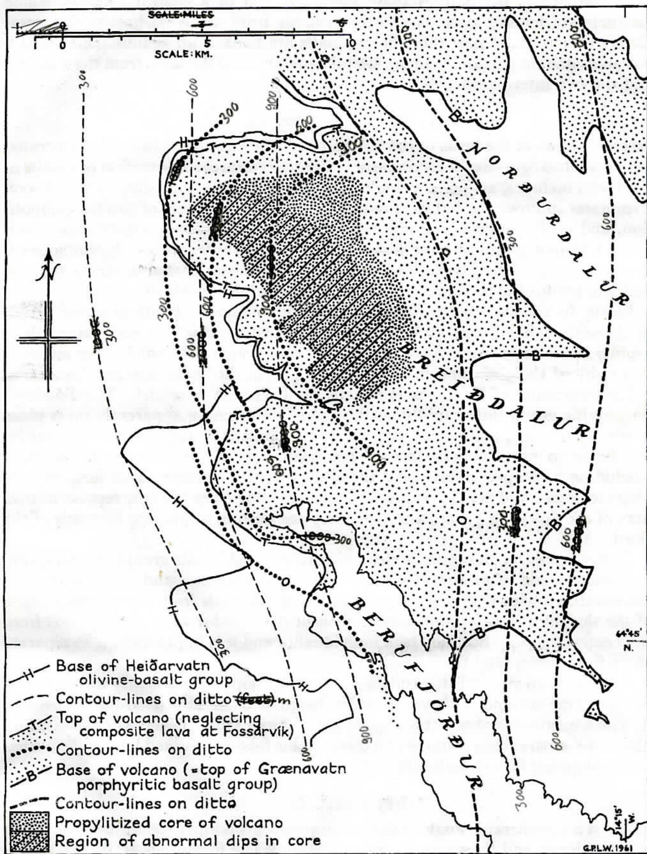
FIG. 5. Structural map of the Breiddalur volcano, with contour-lines drawn on the base and top and on a horizon in the flood-basalts overlapping the volcano.
