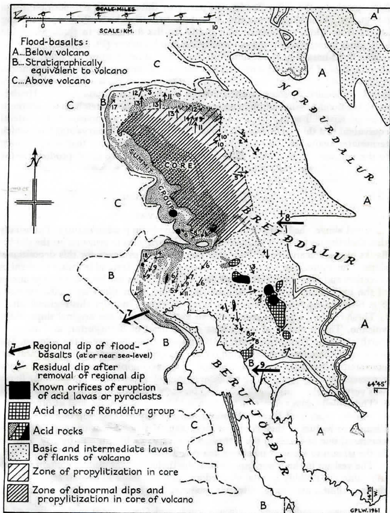
FIG. 6. Simplified geological map of the Breiddalur volcano, showing the probable original depositional dips of the rocks.
