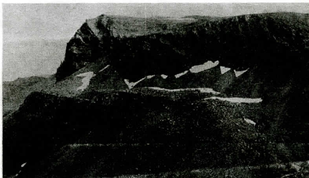
(a) North-western side of Berufjartindur, showing the summit rhyolite flow. Underlying basalts of the summit group on the left.
