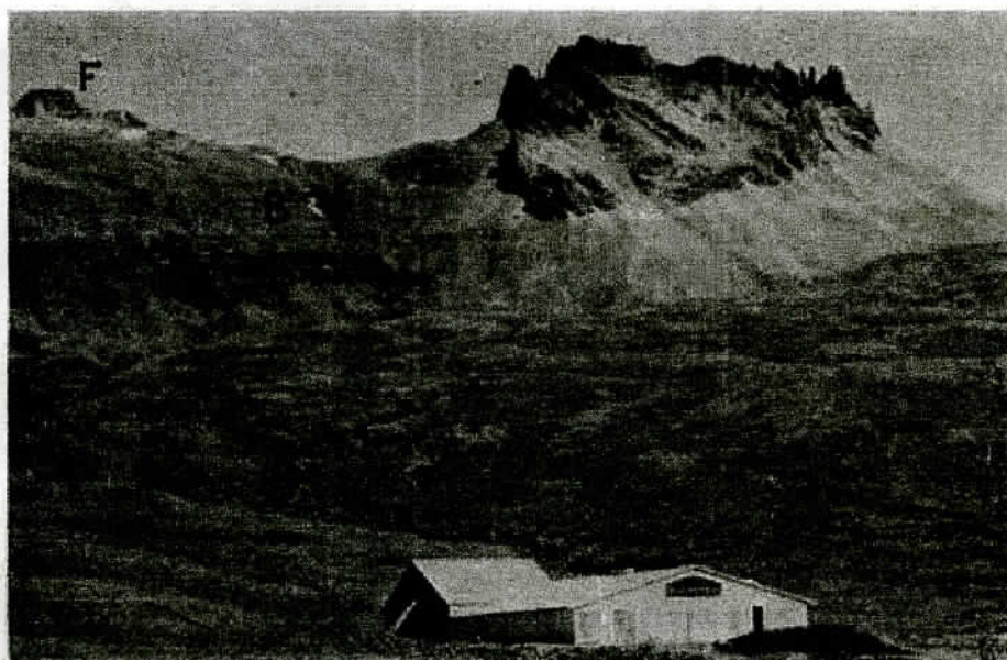
(b) Smátindur from the south-west: rhyolite plug in contact with basalt lavas ( B ).
