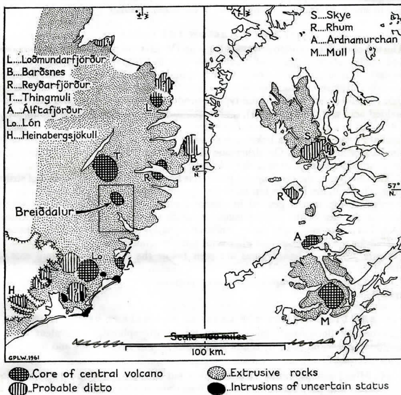
FIG. 1. Index-map of eastern Iceland (left) to show the location of the area described and the positions of other Tertiary volcanic centres. The Hebridean region is shown on the same scale (right) for comparison.
